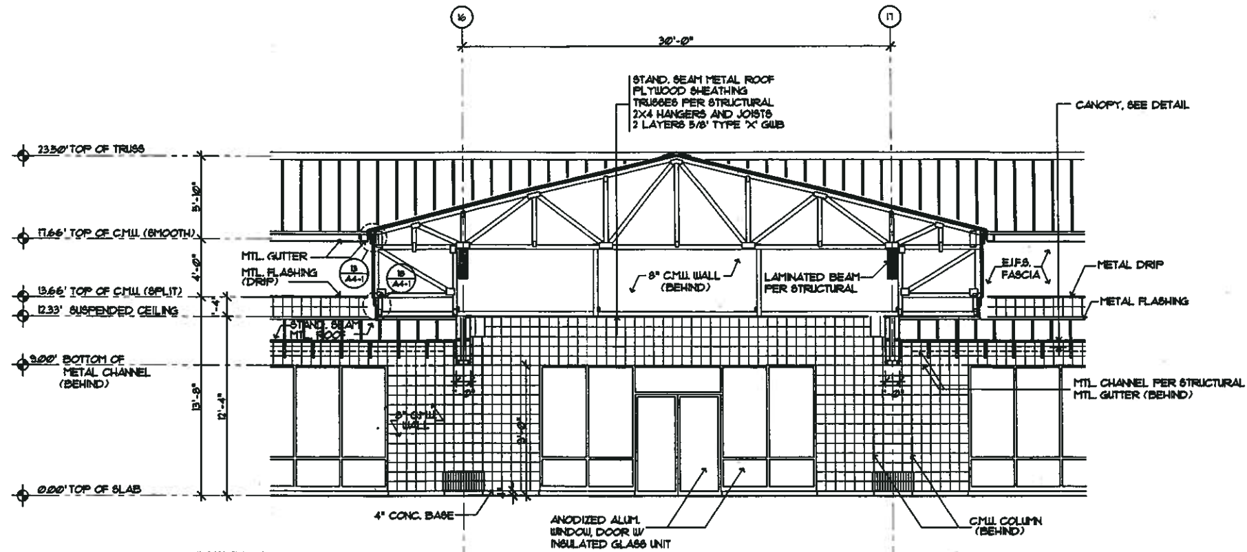
BUILDING SECTION C-C SCALE: 1/4" = 1'-0"
